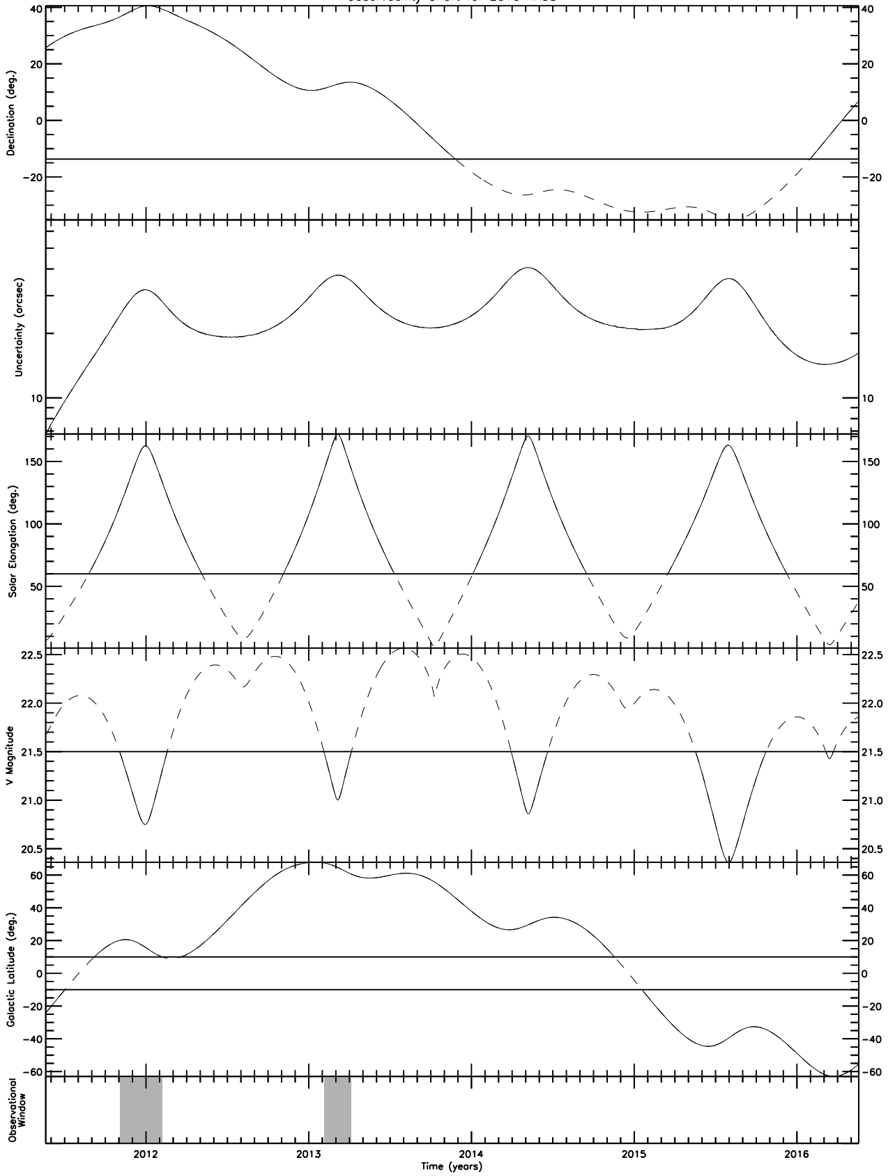
Observability Chart for 2010 RA38
