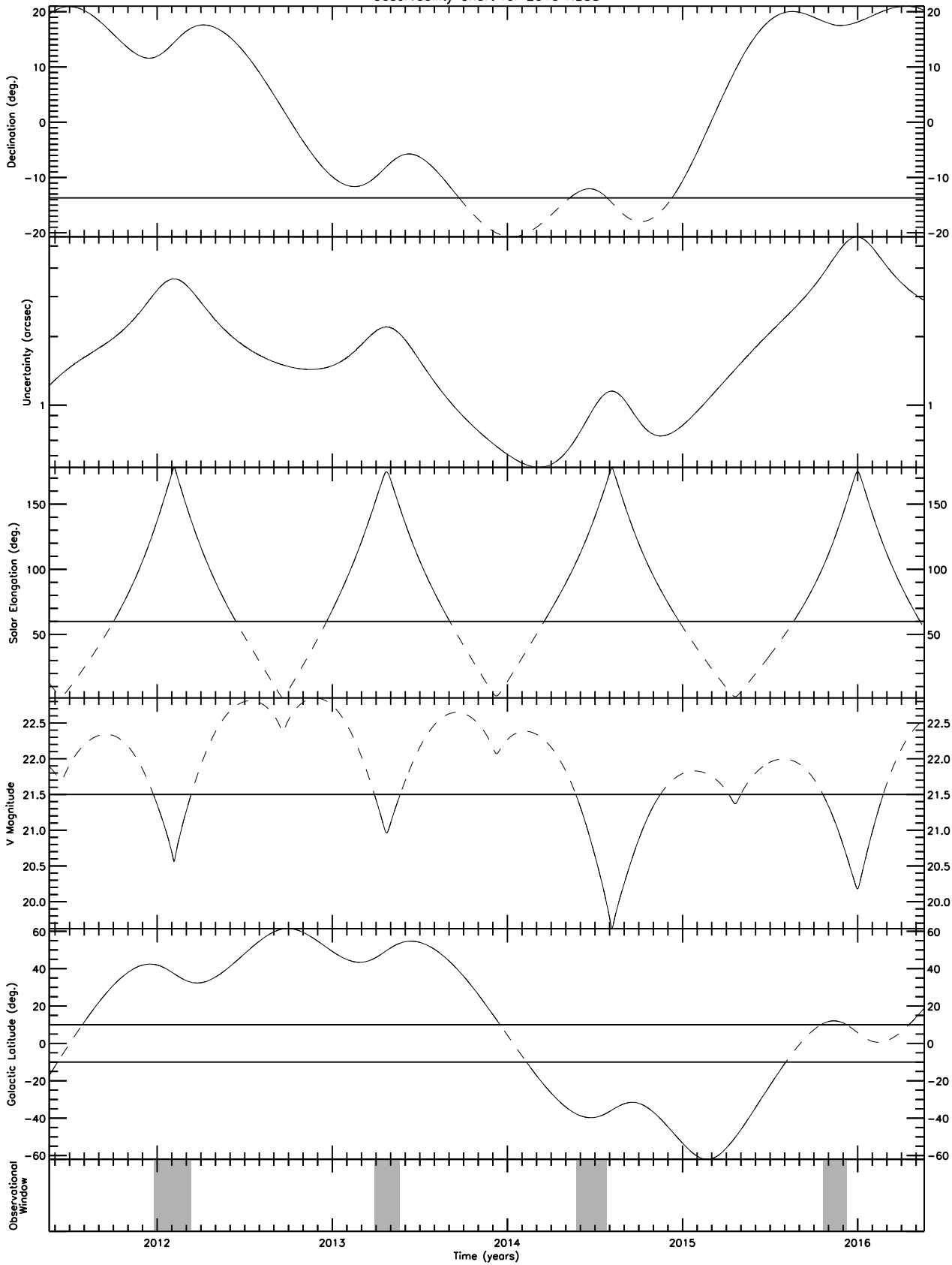
Observability Chart for 2010 RB38
