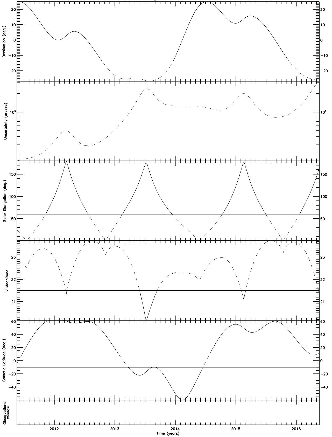
Observability Chart for 2010 RS37
