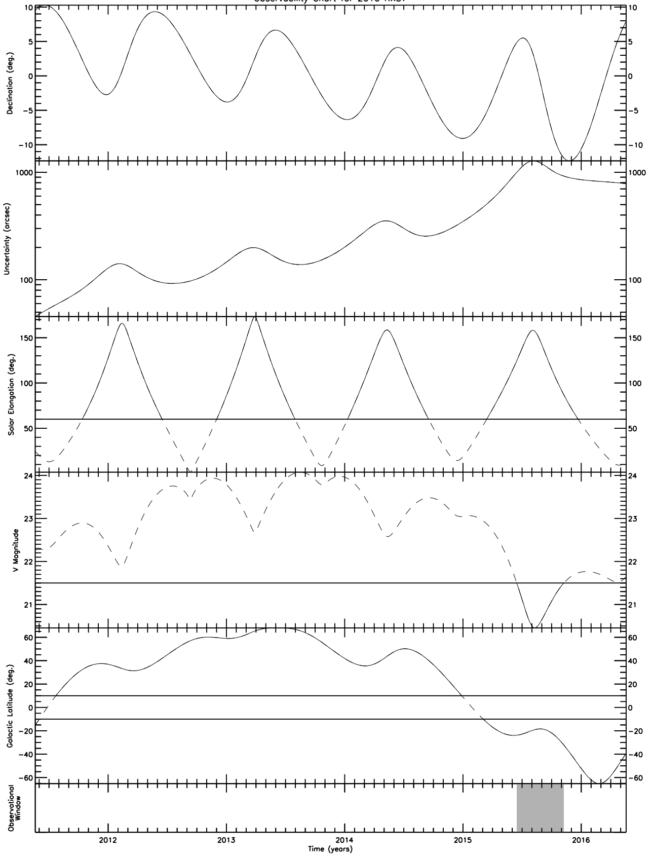
Observability Chart for 2010 RX37
